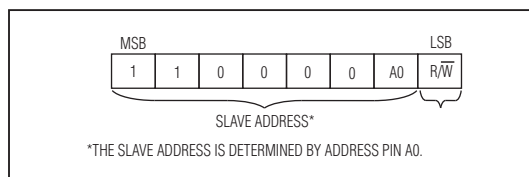
Figure 5. DS3510 Slave Address Byte
